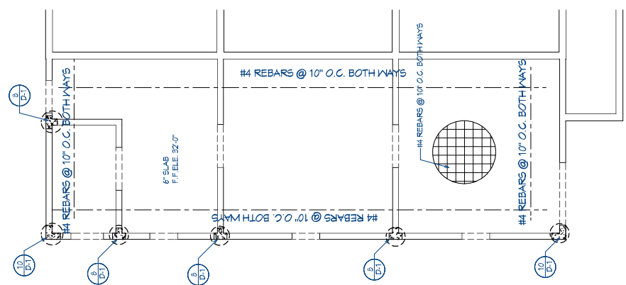
STORAGE LEVEL STRUCTURAL PLAN
