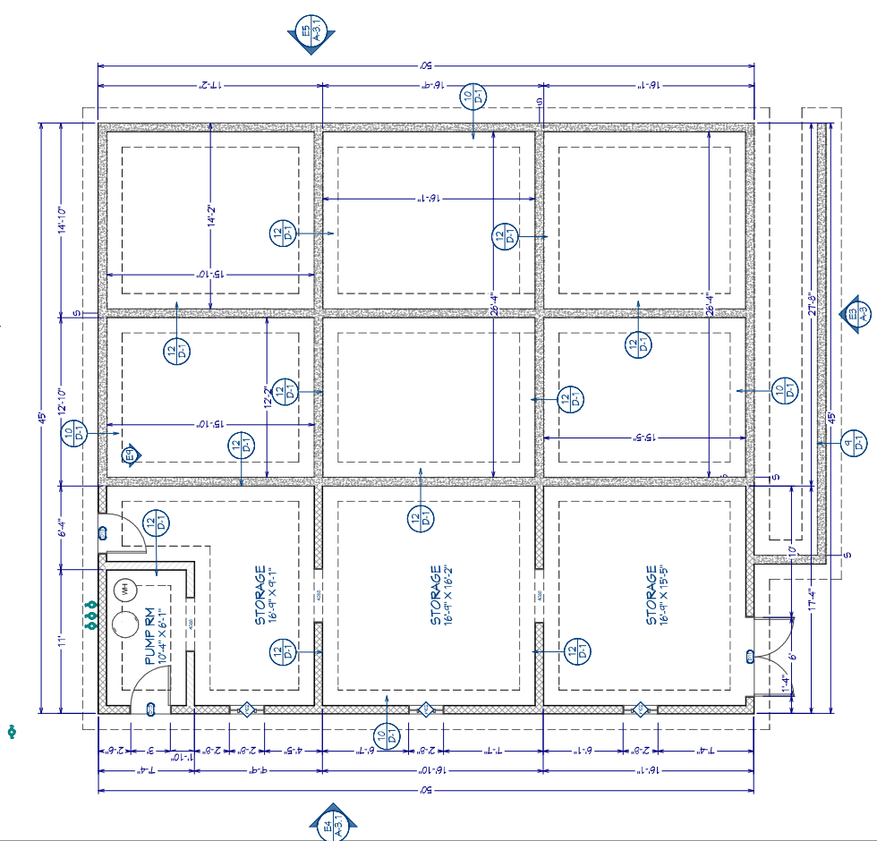
FOUNDATION LEVEL FLOOR PLAN
