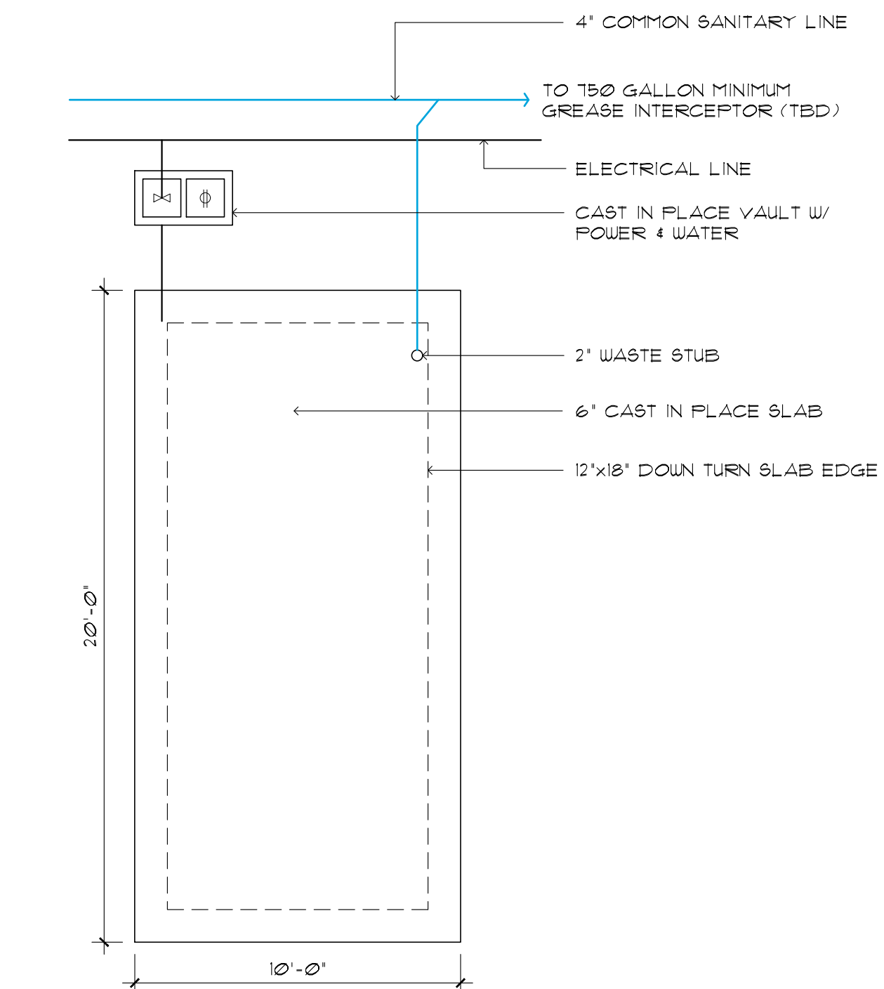
A0.11-3 TYPICAL VENDOR SLAB
