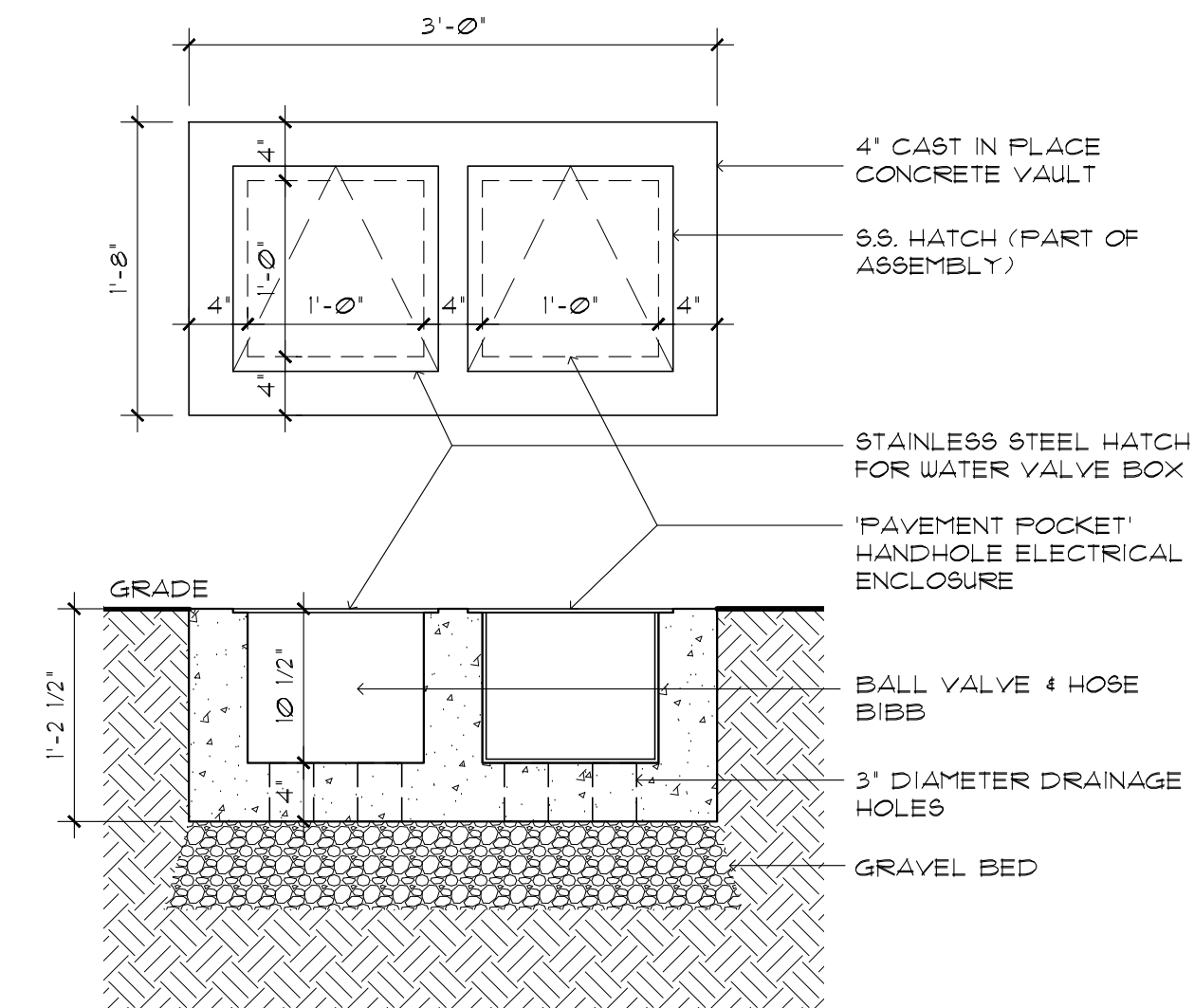
A0.11-3 POWER & WATER VAULT
