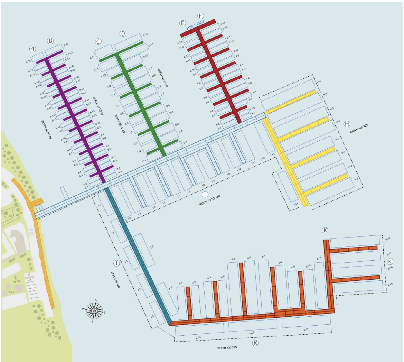
THE YACHT CLUB AT SUMMERS END (YCSE) - BERTH LAYOUT
